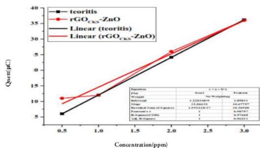
Figure 10. The relation between Q nett and concentration of methylene blue (MB) compound.
