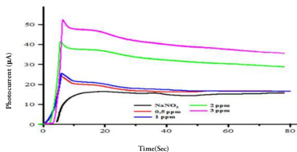
Figure 9. The photocurrent response of methylene blue, amperomogram of rGO PS - ZnO electrode
