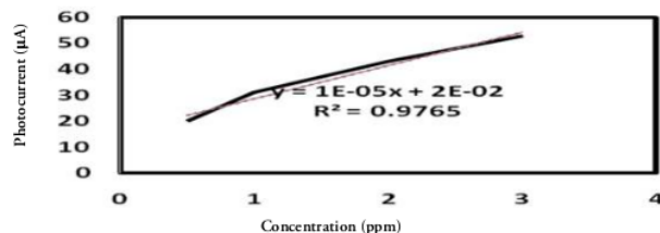
Figure 12. Linear graph of methylene blue test compound
