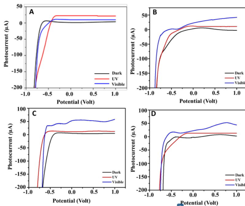
Figure 1. Test of electrode activities by the process of LSV (A) TiO 2 /Ti; (B) S-TiO 2 /Ti 0.5 M; (C) S-TiO 2 /Ti 1 M; and (D) S-TiO 2 /Ti 2 M
