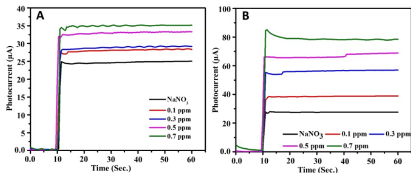
Figure 3. The photocurrent response of phenolic compound (A) Amperomogram of \text{TiO}_2/\text{Ti} electrode; (b) Amperomogram of S- \text{TiO}_2/\text{Ti} electrode
