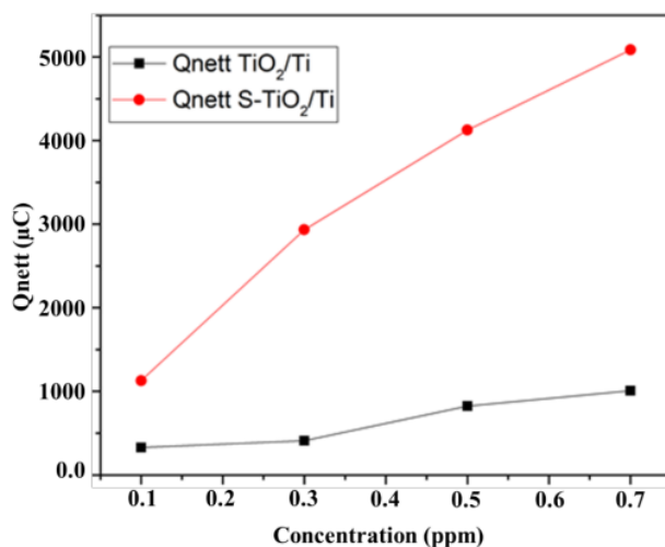
Figure 4. The relation between Q net and concentration of phenolic compound
